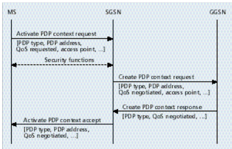
FIGURE 4. PDP context activation.
