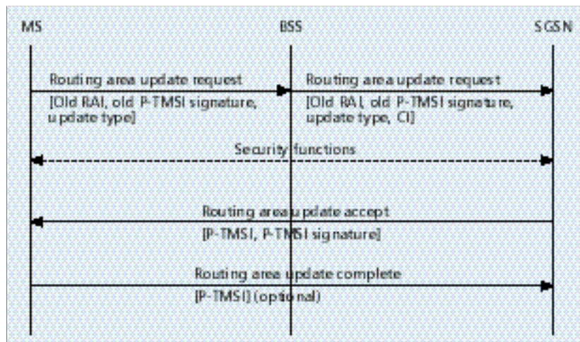
■ FIGURE 6. Intra-SGSN routing area update.
