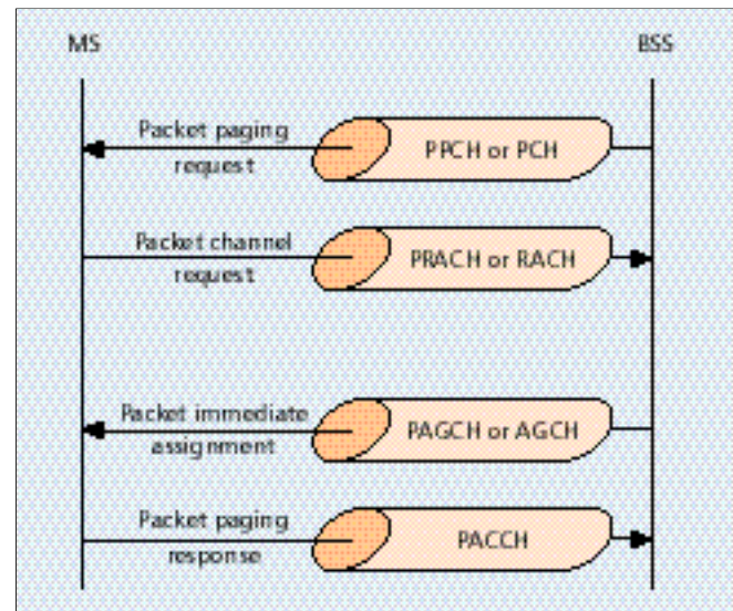
■ FIGURE 9. Paging (mobile terminated packet transfer).
