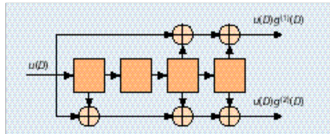
■ FIGURE 12. Convolutional encoder.
