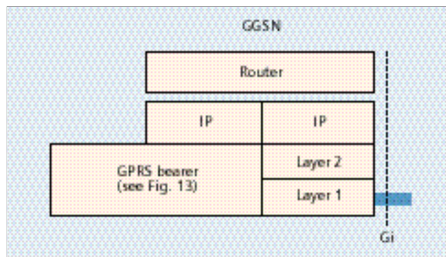
■ FIGURE 17. Protocols at the Gi IP interface.
