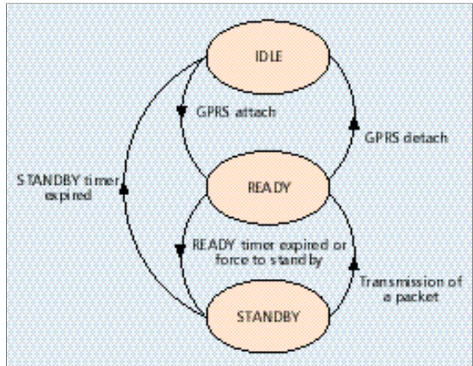
■ FIGURE 5. State model of a GPRS mobile station.
