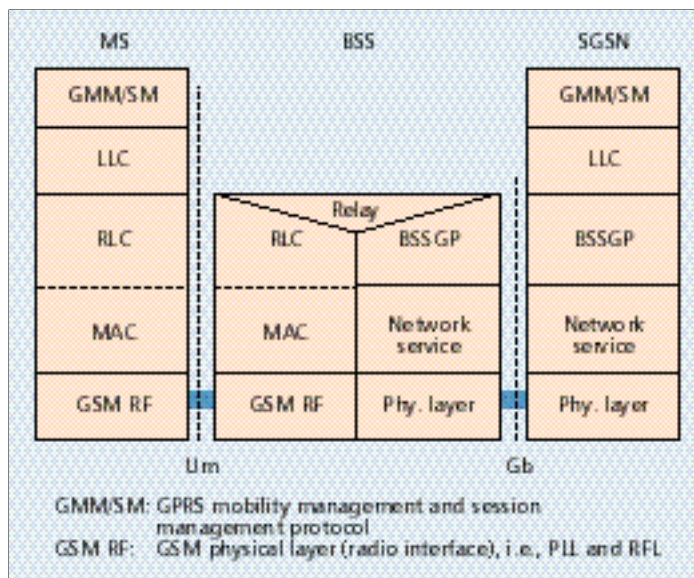
■ FIGURE 14. Signaling plane: MS-SGSN.
