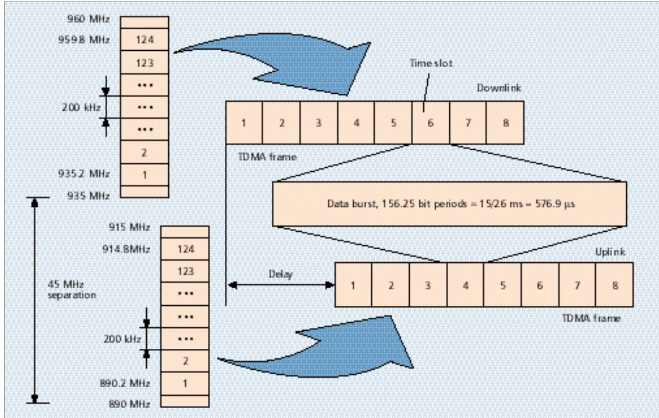
■ FIGURE 7. GSM carrier frequencies, duplexing, and TDMA frames.
