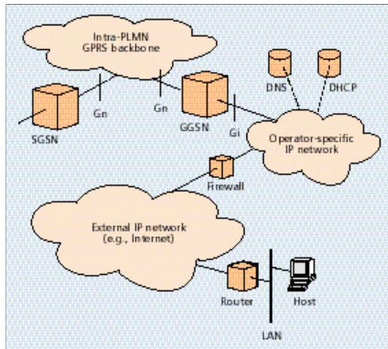
■ FIGURE 18. Example of a GPRS-Internet connection.
