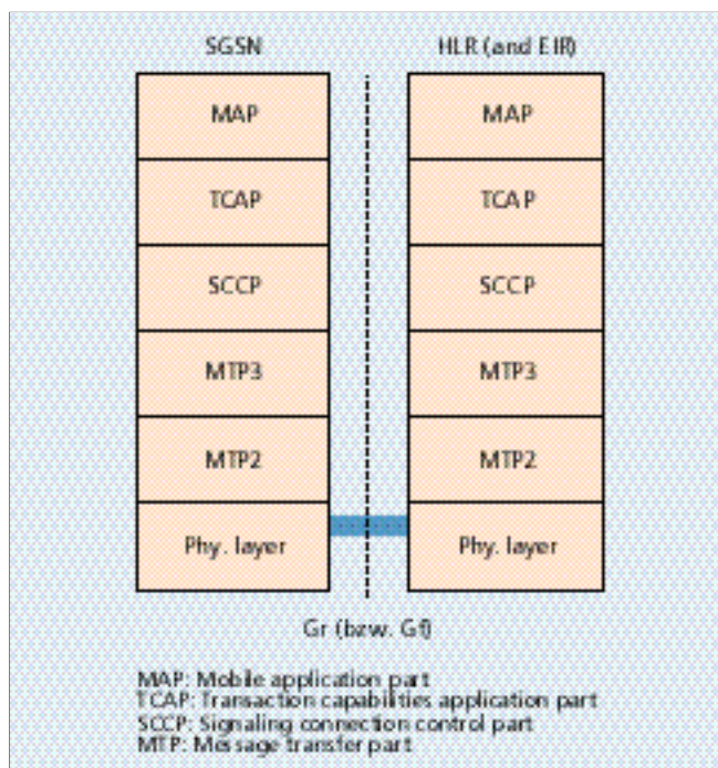
■ FIGURE 15. Signaling plane: SGSN-HLR, SGSN-EIR.
