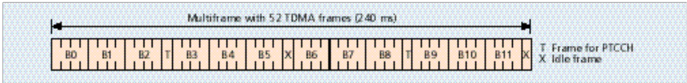
■ FIGURE 10. Multiframe structure with 52 frames.
