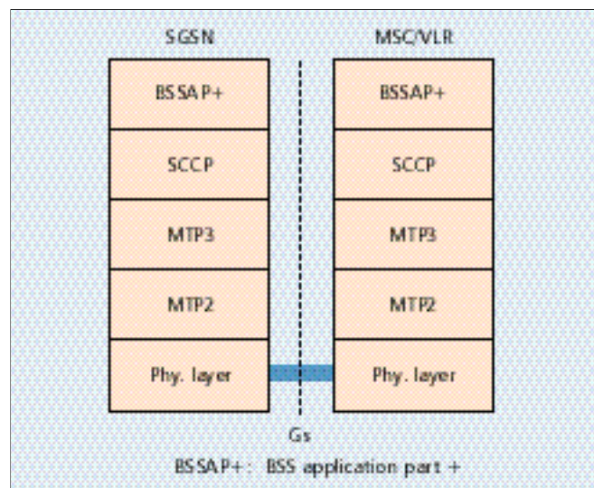
■ FIGURE 16. Signaling plane: SGSN- MSC/VLR.
