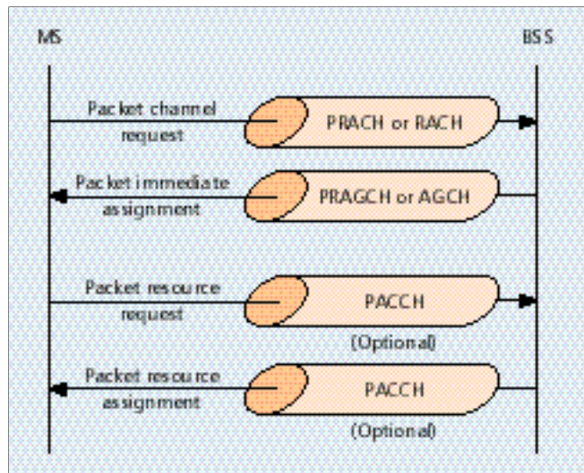
■ FIGURE 8. Uplink channel allocation (mobile originated packet transfer); one or two steps.
