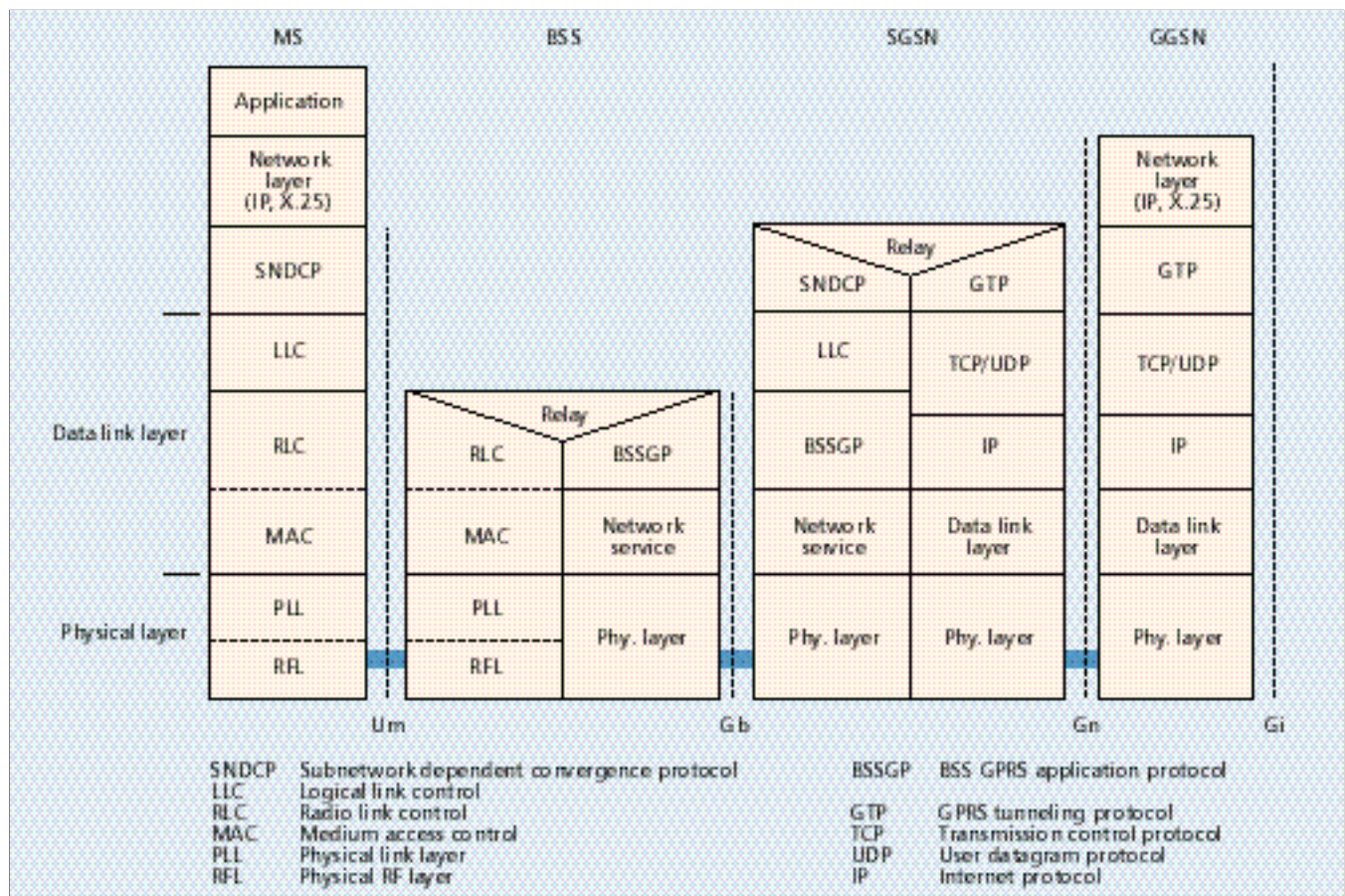
■ FIGURE 13. Transmission plane.
